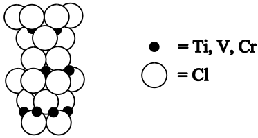
\delta -form \text{MX}_3 catalyst crystal
