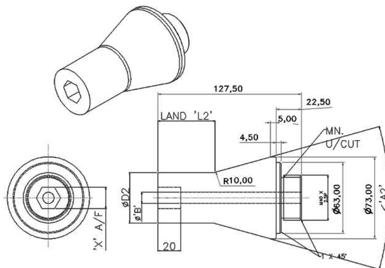
Figure 3.19 Detailed drawing of pin
