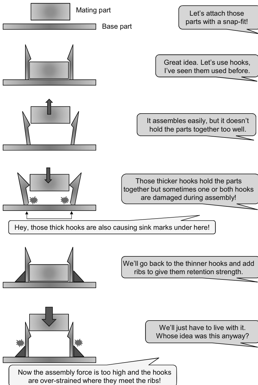
Figure 6.9 Common (bad) hook development scenario
