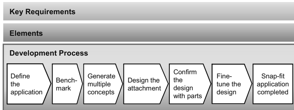
Figure 10.1 The snap-fit development process in the ALC
