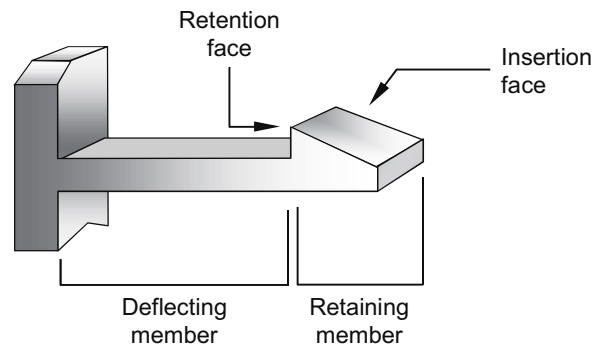
Figure 6.8 The basic hook
