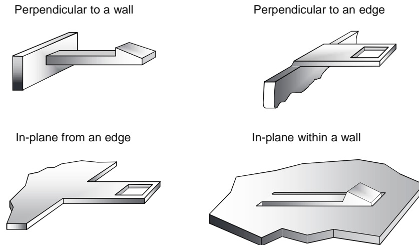
Figure 6.5 Common beam orientation to local part geometry
